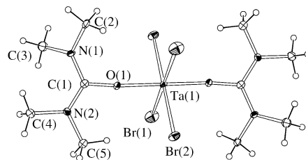
Figure 2. View of the [\text{TaBr}_4(\text{TMU})_2]^+ cation in [\text{TaBr}_4(\text{TMU})_2]_2[\text{TaBr}_6] , 4 . Thermal ellipsoids are drawn at 30% probability level. Only independent atoms are labeled.
