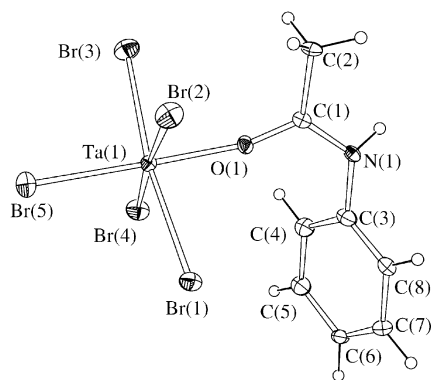
Figure 4. Molecular structure of \text{TaBr}_5(\text{PhA}) , 7b . Thermal ellipsoids are drawn at 30% probability level.
