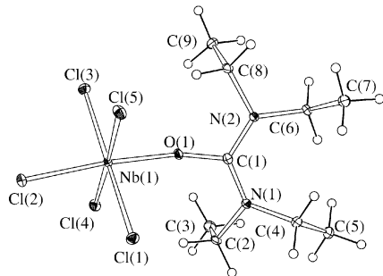
Figure 1. Molecular structure of \text{NbCl}_5(\text{TEU}) , 3a . Thermal ellipsoids are drawn at 30% probability level.
